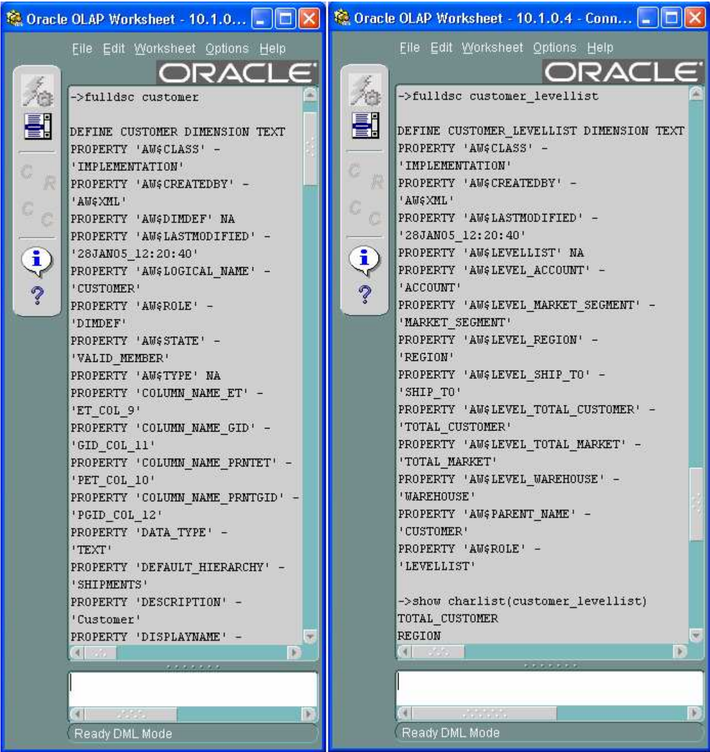
Figure 2 – Metadata Created by AWM
